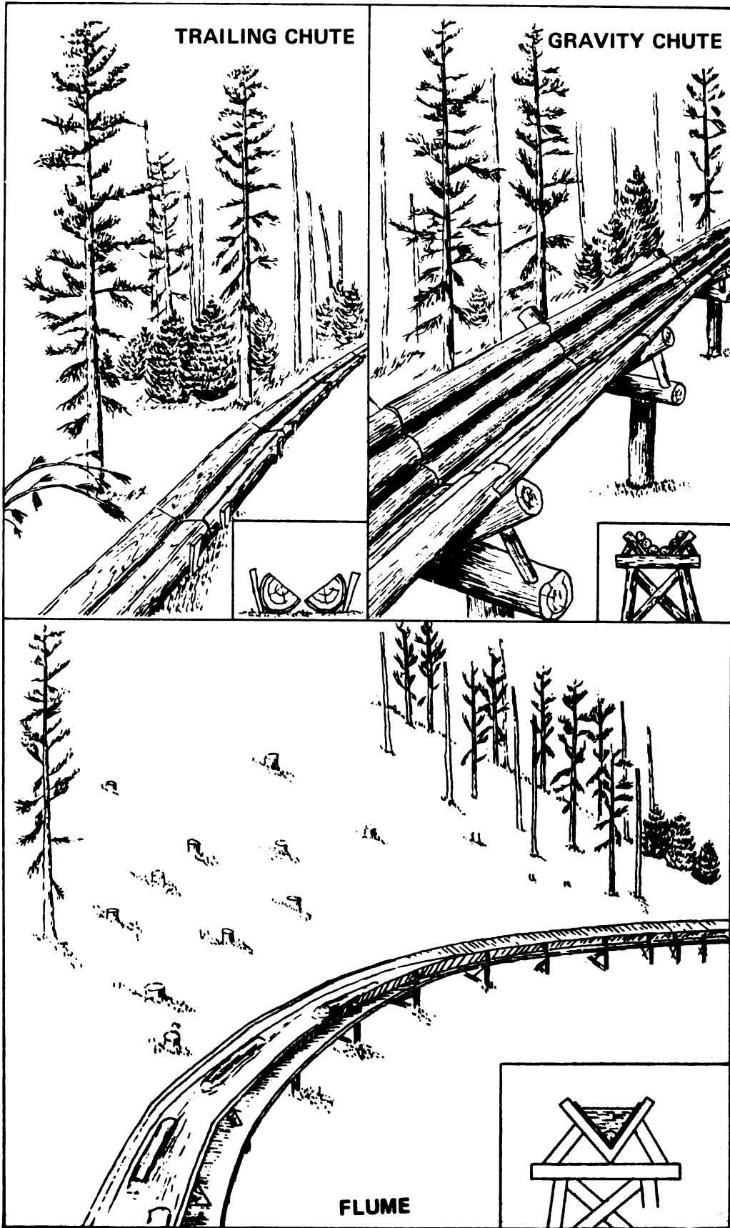
Figure 7-22. Chutes and flumes.
